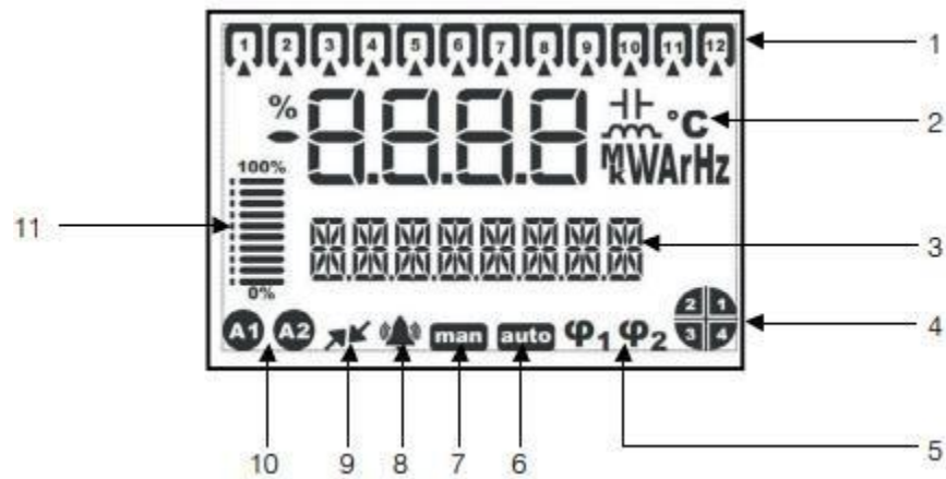
Figura 3. Panel frontal
